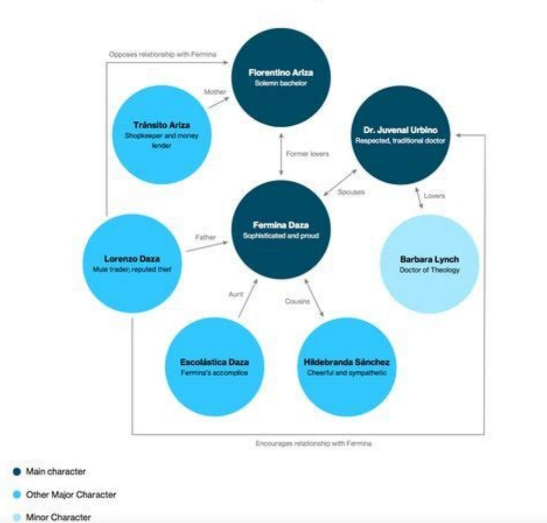
Character Map
